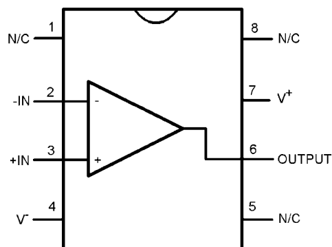
8-Pin SOIC (LMH6642)
