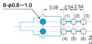
PC Hole Layouts (Top view)
