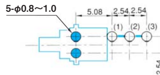
C Hole Layouts (Top view)
