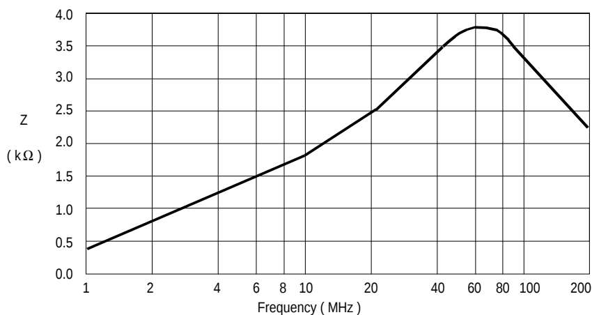
P/N F-1506 Typical Impedance Plot
