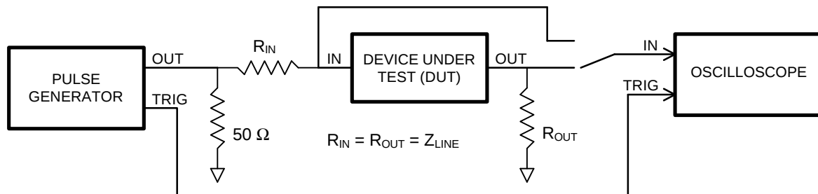
Test Setup
