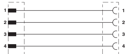
Contact assignment of the DEUTSCH connectors
