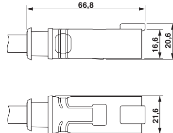
DEUTSCH DT04-4P, top view and side view
