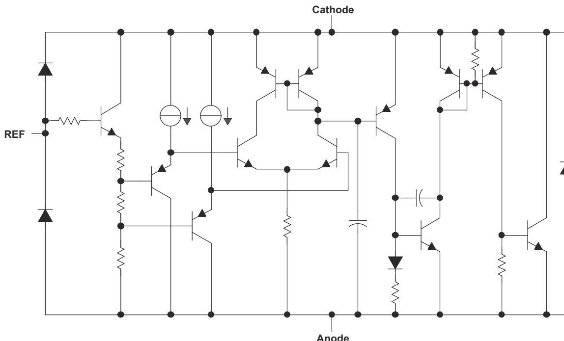
Figure 7-2. Detailed Schematic
