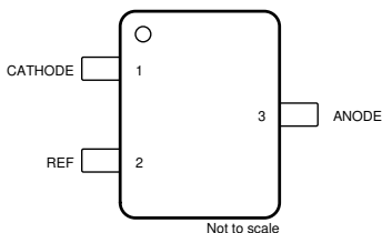
Figure 4-5. TLVH432 DBZ Package 3-Pin SOT-23 Top View
