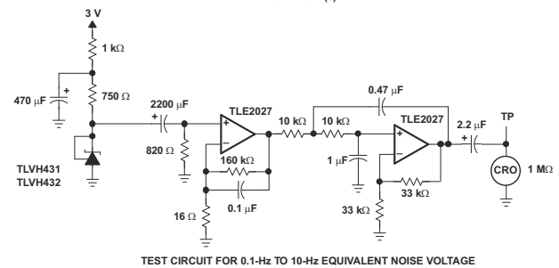
Figure 5-10. Equivalent Input Noise Voltage
