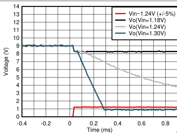
Figure 8-3. Output Response With Small Overdrive Voltages
