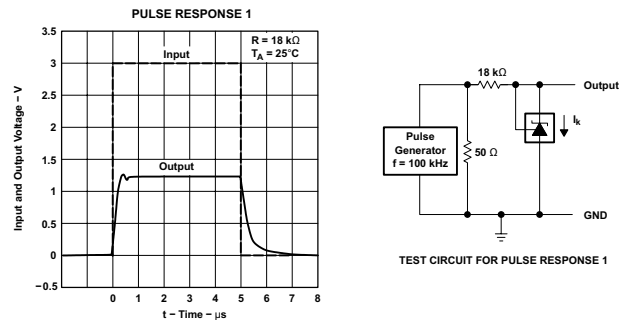
Figure 5-12. Pulse Response 1
