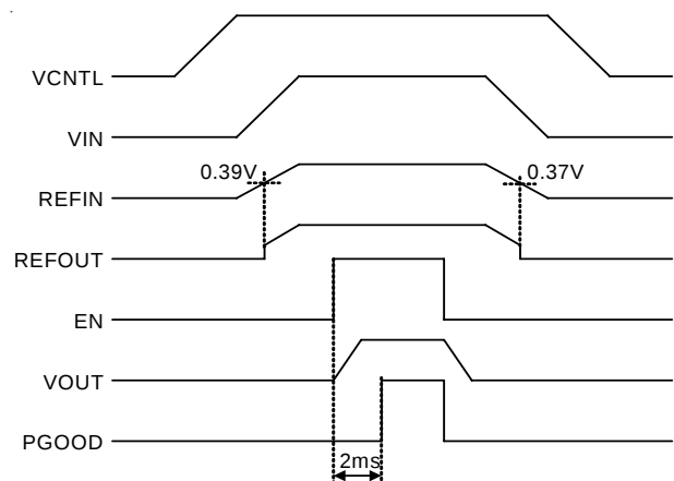
Figure 1. Typical Start Up and Shutdown Timing Diagram
