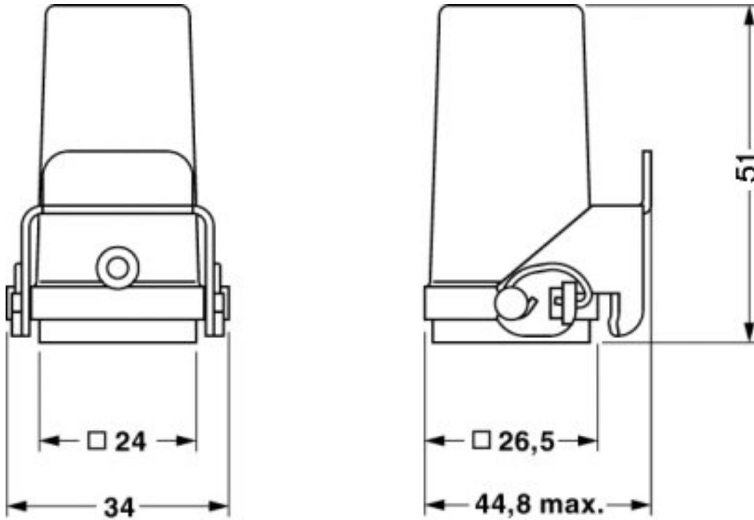
Dimensioned drawing
