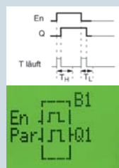
Pulse generator
