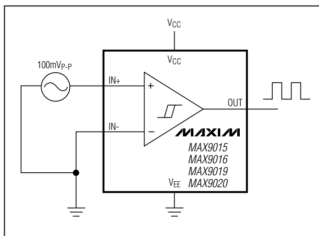
Figure 5. Zero-Crossing Detector
