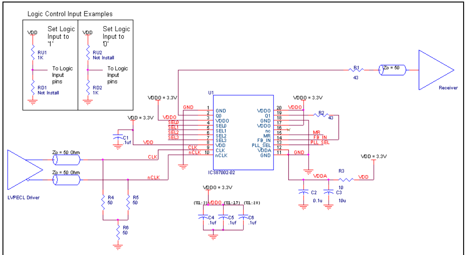
Figure 4. ICS87002-02 Schematic Example
