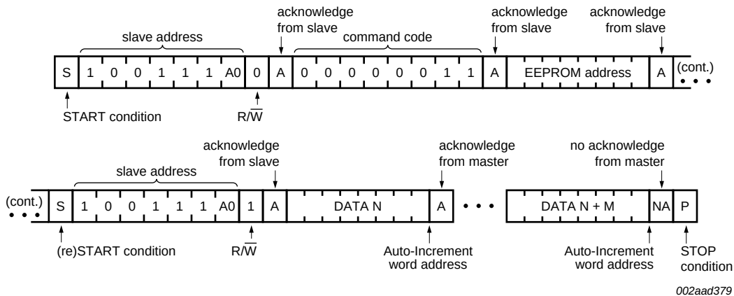
Fig 15. I 2 C-bus read operation from 256-byte EEPROM
