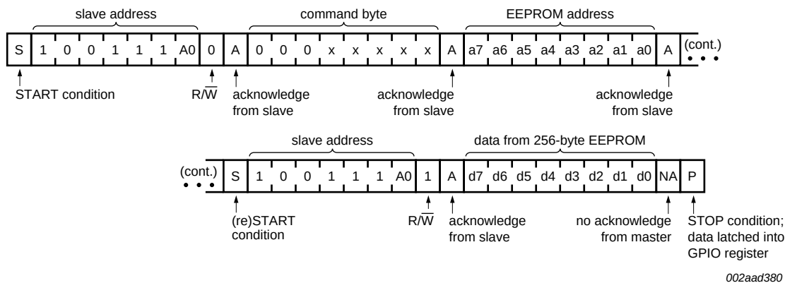
Fig 16. Read from 256-byte EEPROM and write to GPIO registers
