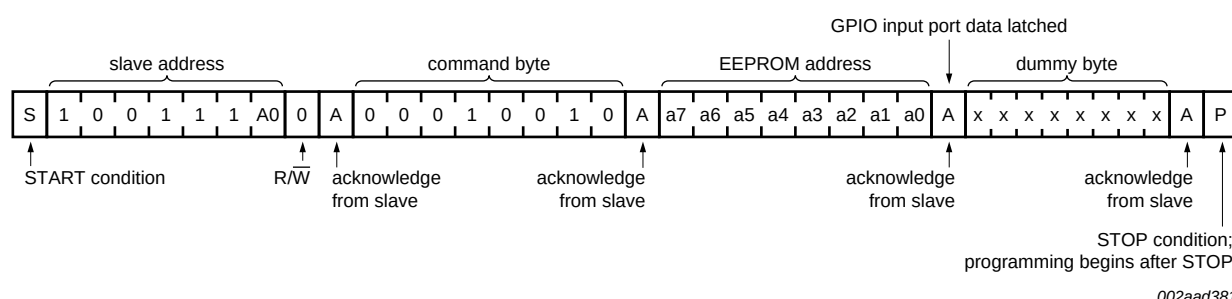
Fig 17. Read from GPIO Input Port register and write to 256-byte EEPROM
