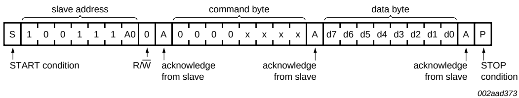
Fig 9. I 2 C-bus write for GPIO registers
