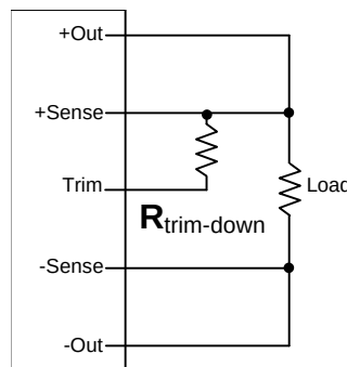
Trim Down
