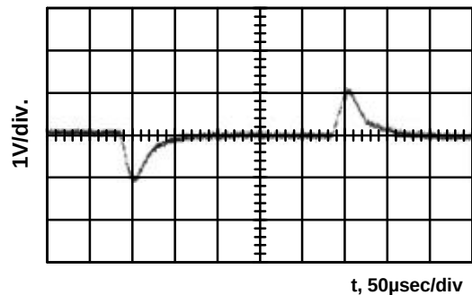
Transient Response
