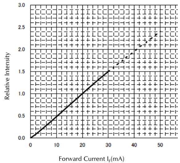
Forward Current vs. Relative Intensity Condition : T_a = 25^\circ\text{C}
