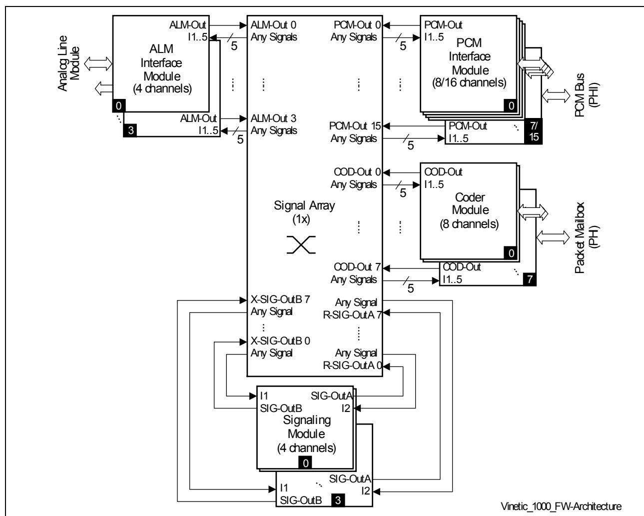
Figure 9 Module Concept
