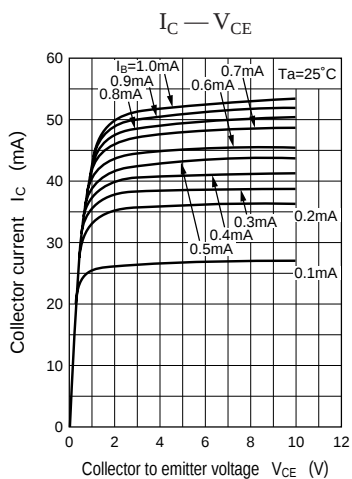
Characteristics charts of UN221E
