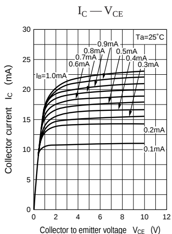
Characteristics charts of UN221D
