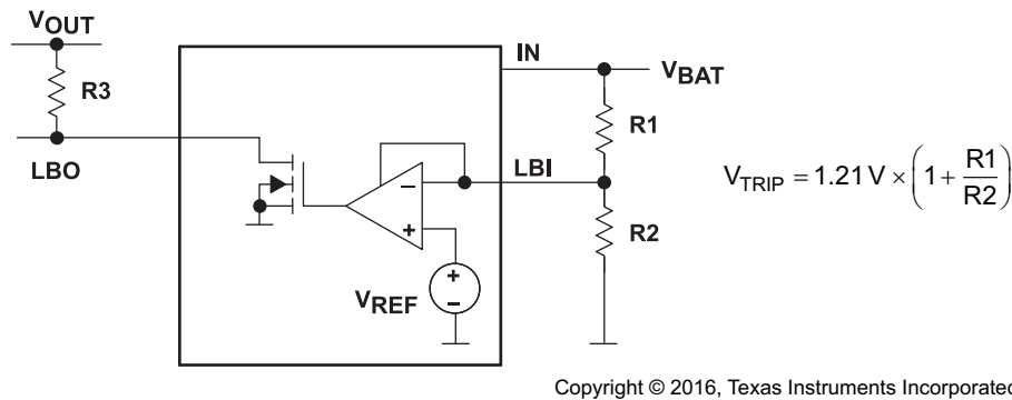
Figure 21. Programming of the Low Battery Comparator Trip Voltage
