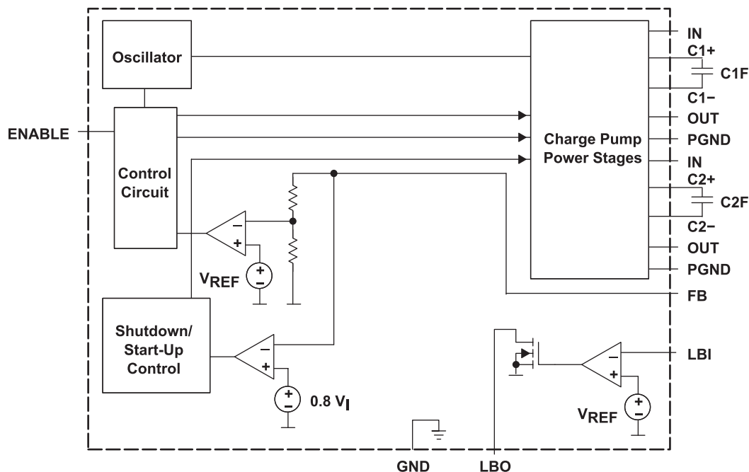
Figure 19. TPS60130 and TPS60132 Block Diagram
