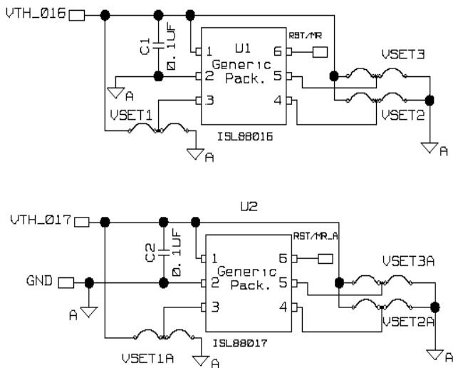
FIGURE 4. ISL88016/17EVAL1Z SCHEMATIC
