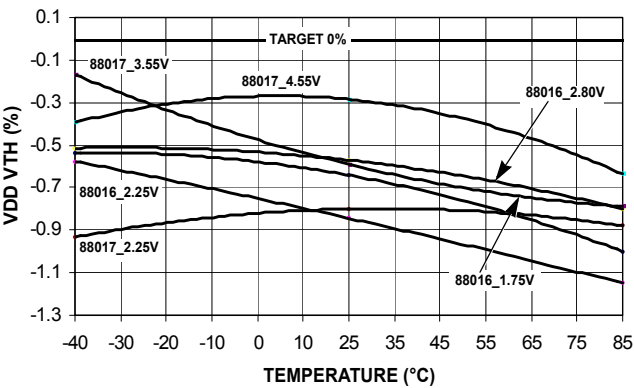
FIGURE 6. SAMPLED V_{\text{TH}}\% TO TARGET OVER TEMP
