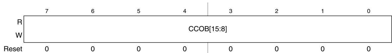
Figure 23-15. Flash Common Command Object High Register (FCCOBHI)
