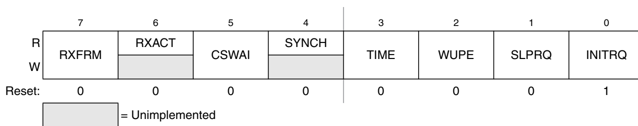
Figure 18-4. MSCAN Control Register 0 (CANCTL0)
