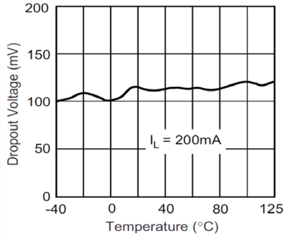
Figure 22. Dropout Voltage
