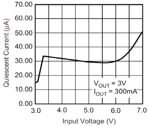
Figure 16. Ground Pin Current
