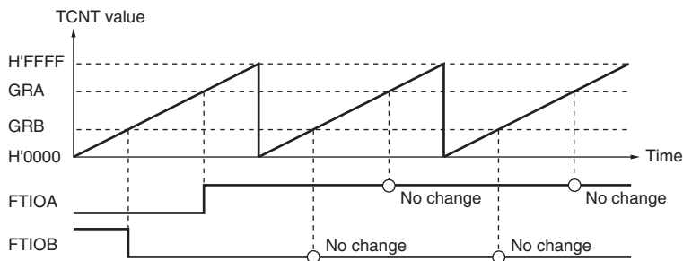
Figure 11.4 0 and 1 Output Example (TOA = 0, TOB = 1)
