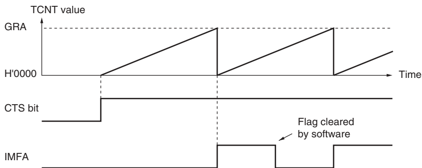
Figure 11.3 Periodic Counter Operation
