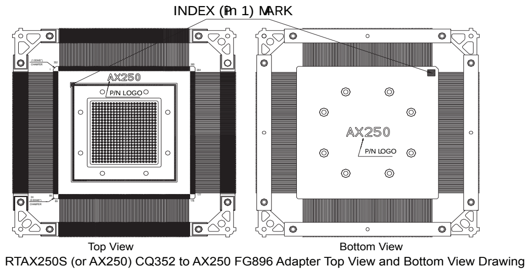
Figure 6 • RTAX250S CQ352 to FG484 Adapter Top View, Bottom View and Orientation Drawing
