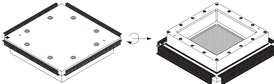
Figure 14 • View of Assembled CQ352 to FG896 Adapter Socket with Socket Housing
