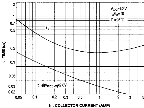
TURN-ON TIME
