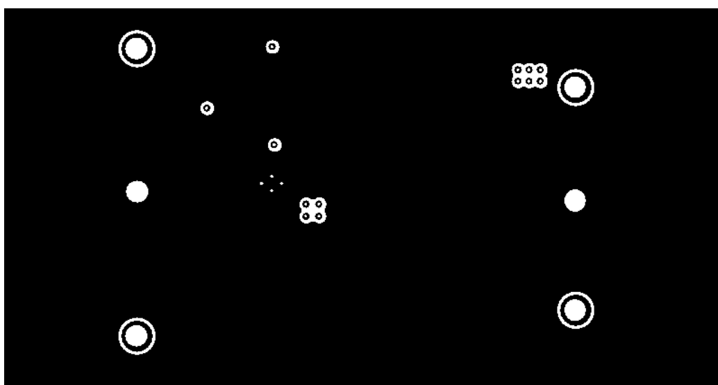
Figure 10. Internal Plane 2
