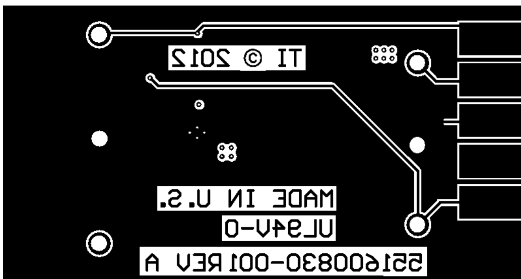
Figure 12. Bottom Copper
