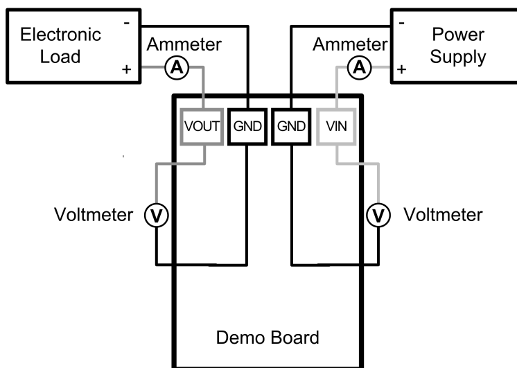
Figure 2. Efficiency Measurements
