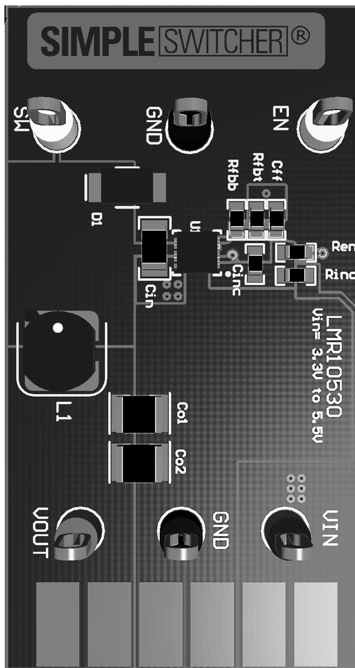
Figure 5. Top Side
