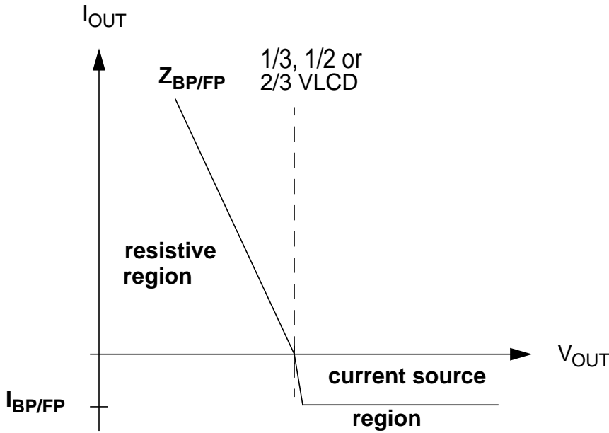
Figure A-7. buffer output characteristic
