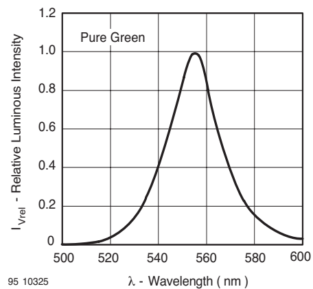
Figure 28. Relative Intensity vs. Wavelength
