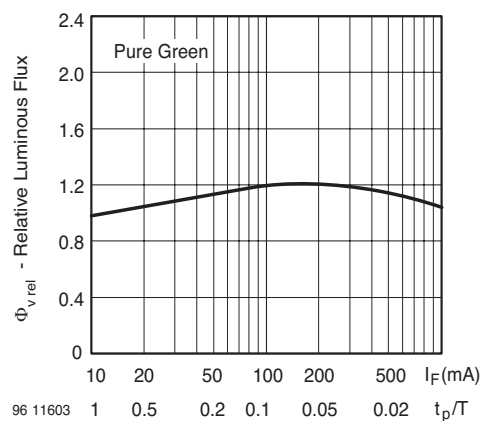
Figure 26. Rel. Luminous Flux vs. Forw. Current/Duty Cycle
