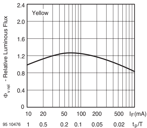
Figure 16. Rel. Luminous Flux vs. Forw. Current/Duty Cycle
