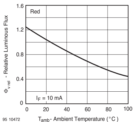
Figure 5. Rel. Luminous Flux vs. Ambient Temperature
