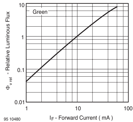
Figure 22. Relative Luminous Flux vs. Forward Current
