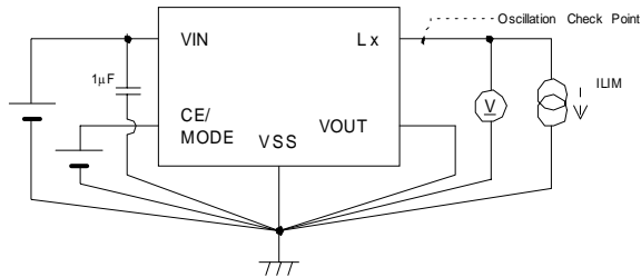
Circuit ⑦
