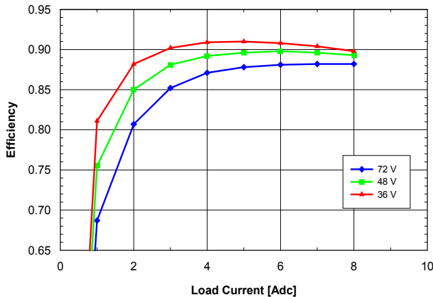
Fig. 6.0V.5: Efficiency vs. load current and input voltage for SQ48T/S08060 converter mounted vertically with air flowing from pin 3 to pin 1 at a rate of 300 LFM (1.5 m/s) and T_a = 25^{\circ}C .
