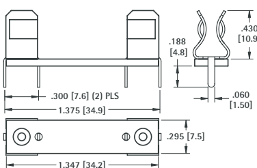
Mounting Detail
