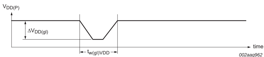
Fig 23. Glitch width and glitch height
