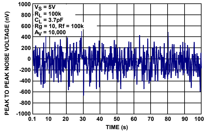
FIGURE 8. INPUT NOISE VOLTAGE 0.01Hz TO 10Hz
