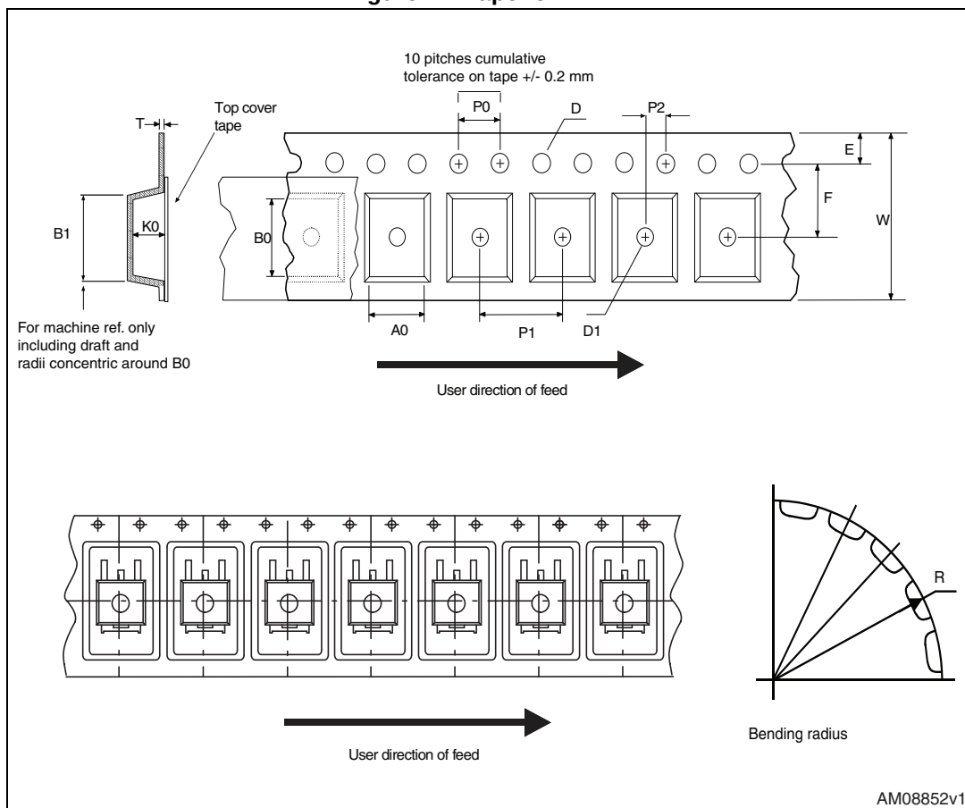
Figure 22. Tape for DPAK
