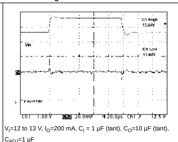
Figure 17. Line transient
