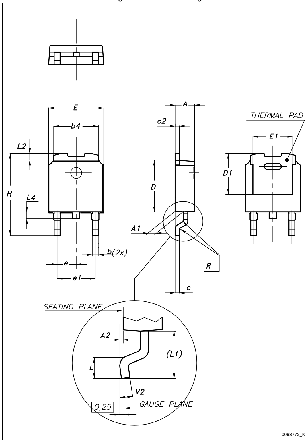
Figure 20. DPAK drawing
