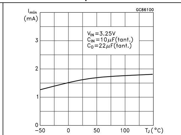
Figure 15. Minimum load current vs temperature
