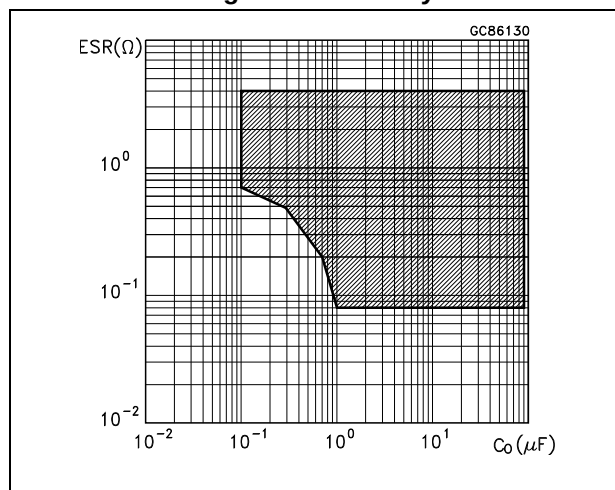
Figure 16. Stability
