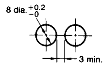
Panel cutout
