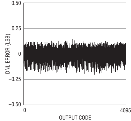
LTC2156-12: Differential Nonlinearity (DNL)
