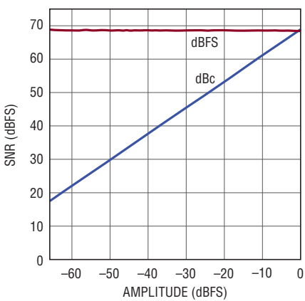
LTC2155-12: SNR vs Input Level, f_{IN} = 70\text{MHz} , 1.5V Range, 170Msps
