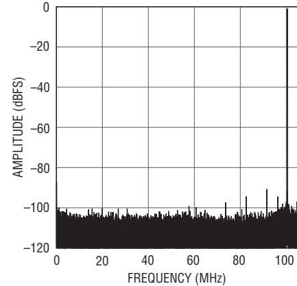
LTC2156-12: 32K Point FFT, f_{IN} = 101\text{MHz} , -1dBFS, 210MSPs
