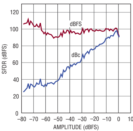
LTC2155-12: SFDR vs Input Level, f_{IN} = 70\text{MHz} , 1.5V Range, 170Msps
