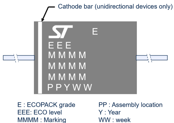
Figure 14. Marking layout
