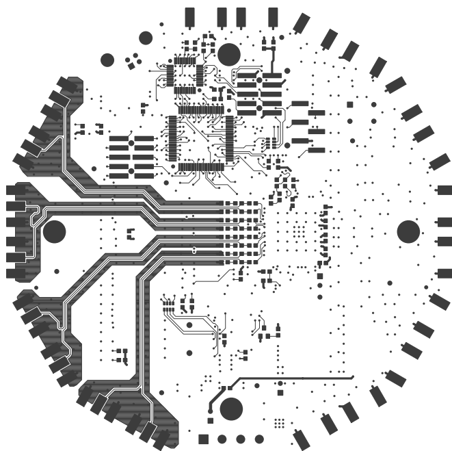
Figure 18. Layer 8
