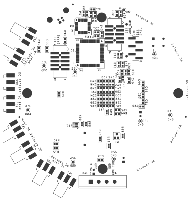
Figure 19. Silkscreen Bottom
