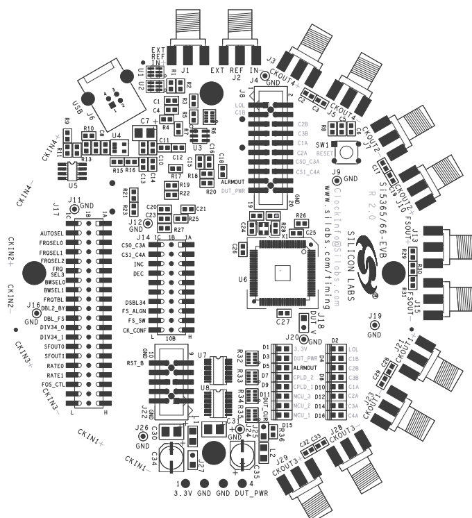
Figure 10. Silkscreen Top
