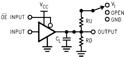
FIGURE 1. AC Test Circuit
