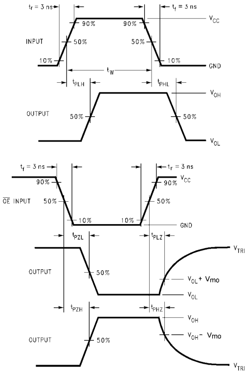
FIGURE 2. AC Waveforms
