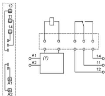
(1) Protection circuit
