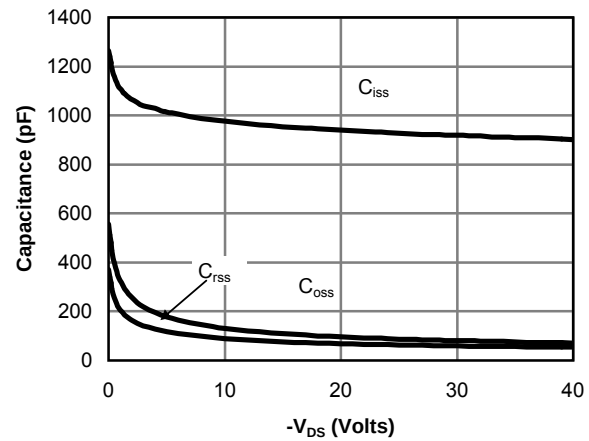
Figure 19: Capacitance Characteristics
