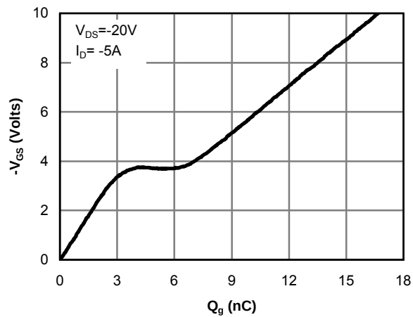
Figure 18: Gate-Charge Characteristics
