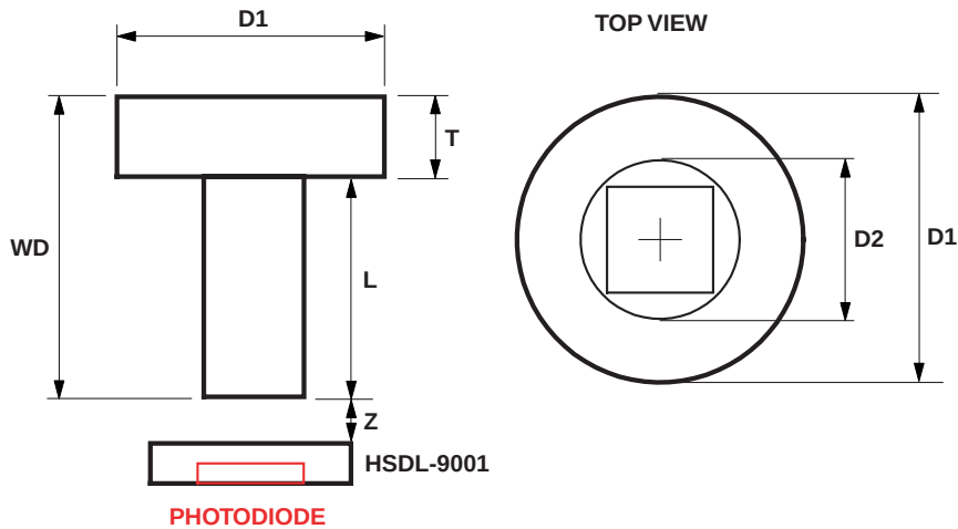
Figure 13. Recommended window dimensions.
