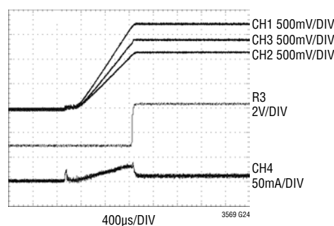
Soft-Start Into Light Load, PS, V_{IN} = 3.6\text{V} , CH1 = V_{OUT1} , CH2 = V_{OUT2} , CH3 = V_{OUT3} , CH4 = I_{IN} , R3 = PG00D
