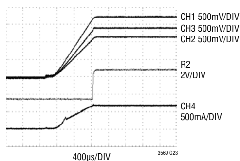
Soft-Start Into Heavy Load, PS, V_{IN} = 3.6\text{V} , CH1 = V_{OUT1} , CH2 = V_{OUT2} , CH3 = V_{OUT3} , CH4 = I_{IN} , R2 = PG00D
