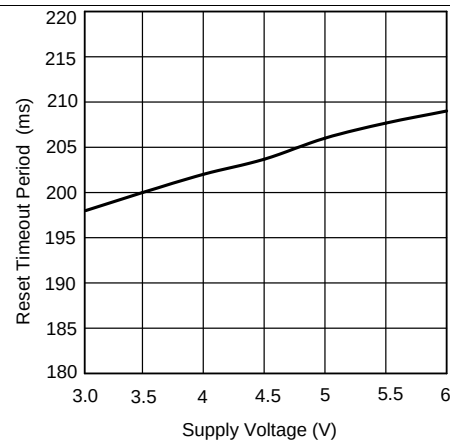
Figure 7. Reset Timeout Period vs V_{CC}
