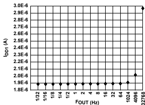
FIGURE 6. I DD1 vs F OUT AT V DD = 5V
