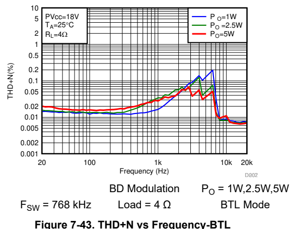
Figure 7-43. THD+N vs Frequency-BTL
