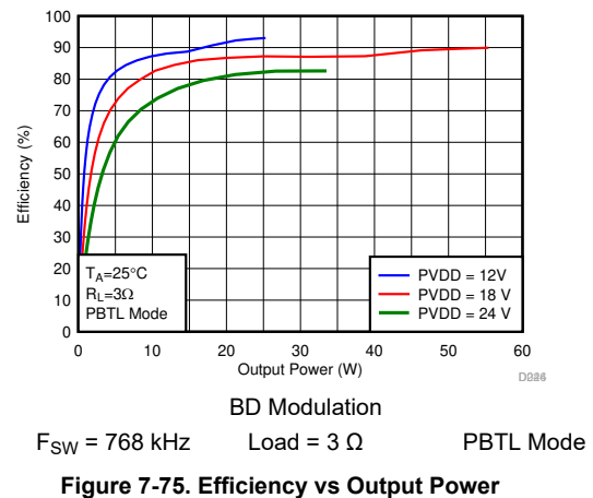
Figure 7-75. Efficiency vs Output Power
