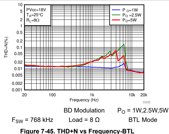
Figure 7-45. THD+N vs Frequency-BTL
