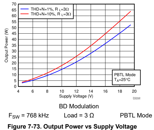
Figure 7-73. Output Power vs Supply Voltage
