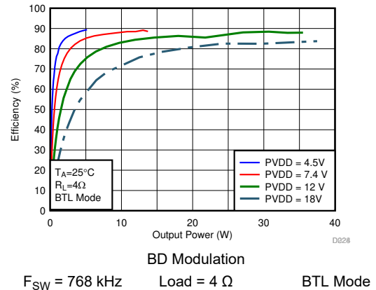
Figure 7-61. Efficiency vs Output Power
