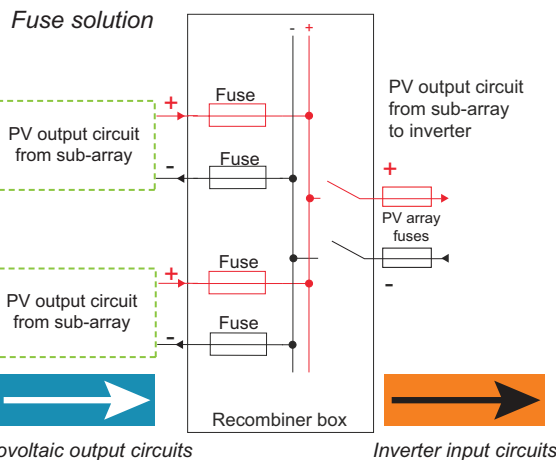
Figure 5: PV output circuit protection (array protection) with NEC® defined circuits designated by arrows.
