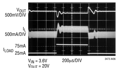
Transient Response
