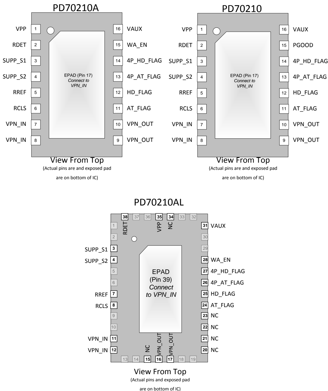
Figure 2: Pinout
