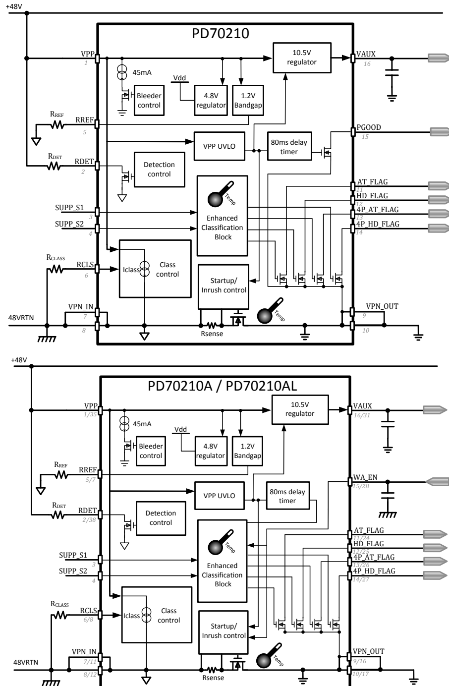
Figure 3: Block Diagram
