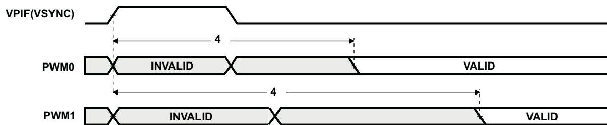
Figure 6-92. PWM Output Delay Timing
