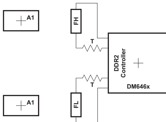
Figure 6-33. DQGATE Routing
