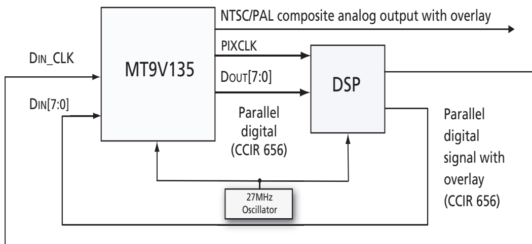
Figure 3: Typical Usage Configuration with Overlay
