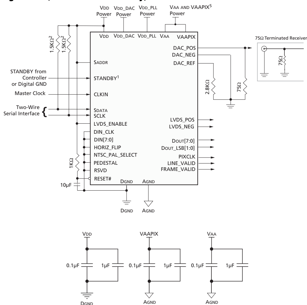
Figure 4: Typical Configuration (without use of overlay)
