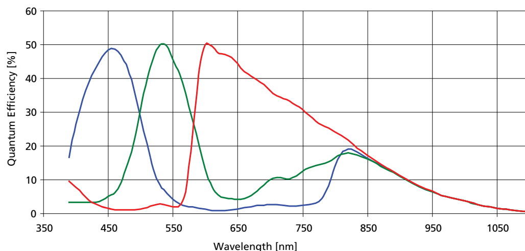
Figure 1: MT9V135 Quantum Efficiency vs. Wavelength
