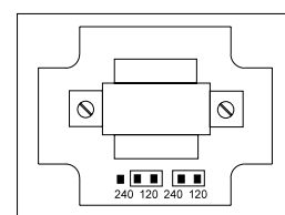
120 VAC Operation
