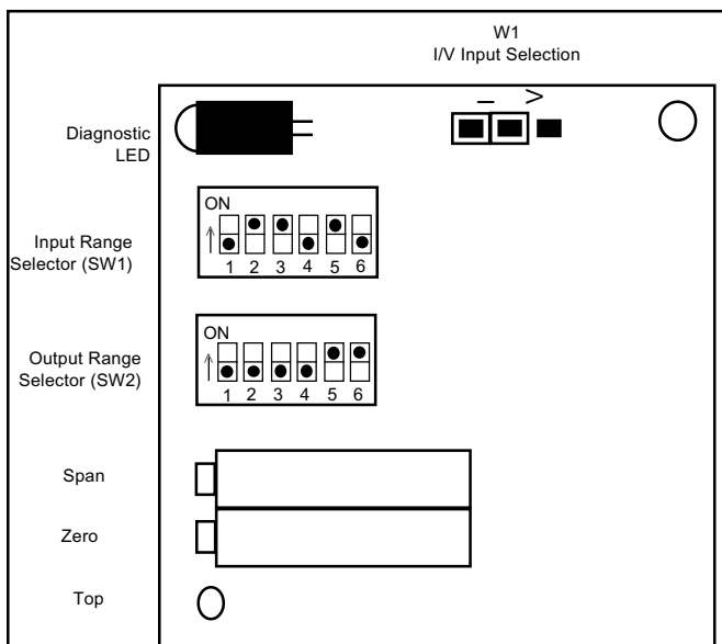
Figure 1: AP4380-2000 I/O card factory calibration: 4-20mA input and output(shown sideways to view switches)
